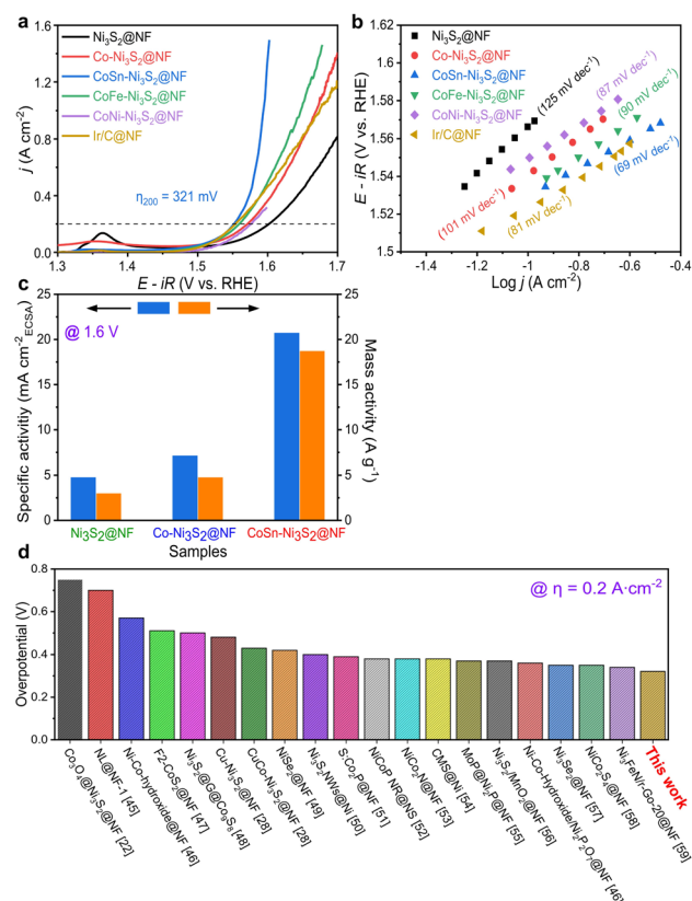
Fig. 4 Electrochemical properties of catalysts for OER. (a) OER polarization curves and (b) Tafel plots of Ni 3 S 2 @NF and T-Ni 3 S 2 @NF with Ir/C@NF. (c) Specific activities and mass activities of Ni 3 S 2 @NF, Co-Ni 3 S 2 @NF, and CoSn-Ni 3 S 2 @NF. (d) Comparison of \eta at 0.2 A cm -2 for CoSn-Ni 3 S 2 @NF with previously reported results for other nickel-based catalysts.
