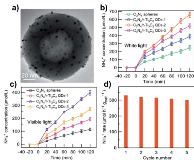
Fig. 14 (a) TEM image of \text{C}_3\text{N}_4/\text{r}-\text{Ti}_3\text{C}_2 QDs-2; (b and c) \text{N}_2 photo-fixation over the different as-obtained photocatalysts. Time courses of the ammonia concentrations measured under white light illumination (light intensity: 300 \text{ mW cm}^{-2} and \lambda = 300\text{--}780 \text{ nm} ) and visible light illumination (light intensity: 300 \text{ mW cm}^{-2} and \lambda = 420\text{--}780 \text{ nm} ); (d) stability tests of \text{C}_3\text{N}_4/\text{r}-\text{Ti}_3\text{C}_2 QDs-2 for \text{N}_2 photofixation under white light. Reproduced with permission from ref. 162, Copyright 2022 The Royal Society of Chemistry.
