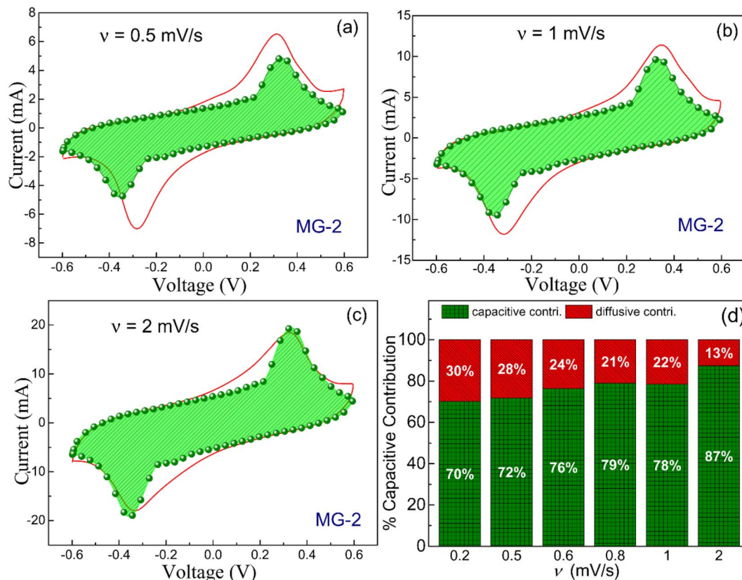
Fig. 13 Dunn method analysis of the capacitance contribution for (a) v = 0.5 , (b) v = 1 , (c) v = 2 \text{mV s}^{-1} , and (d) histogram showing the capacitance contributions of capacitive and diffusive processes at different scan rates for MG-2 nanohybrid.
