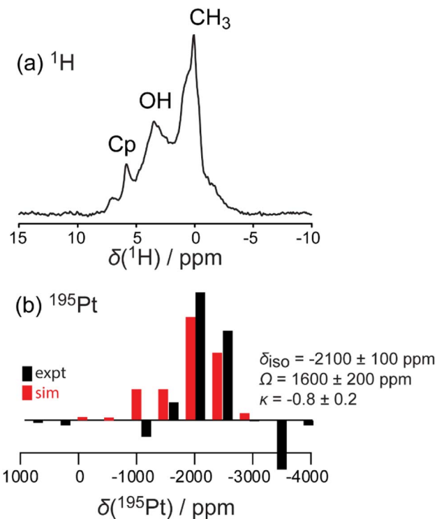
Fig. 6 Simulated (red) and experimental (black) ^1\text{H} MAS (a) and ^1\text{H} ( ^{195}\text{Pt} ) perfect-echo RESPOR (b) solid-state NMR spectra acquired on a MeCpPtMe _3 /STO material.
