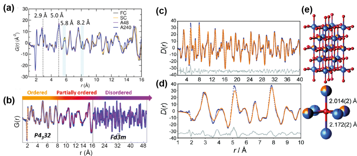
Fig. 12 (a) PDFs of ordered and disordered polymorphs of LiMnNiO 4 . (b) Fitted PDF of the disordered sample with sections showing the regions of the PDF that differentiate the samples. Reprinted with permission from ref. 71. Copyright 2016 American Chemical Society. (c and d) Neutron PDF data for an ordered slow-cooled sample of Li 1.25 Nb 0.25 Mn 0.5 O 2 that has been fitted using a structural model based on the unit cell of \gamma -LiFeO 2 . (e) The O coordination environment is shown (bottom-right) along with the two axial bond lengths. 77 Reproduced from ref. 77 with permission from the Royal Society of Chemistry.
