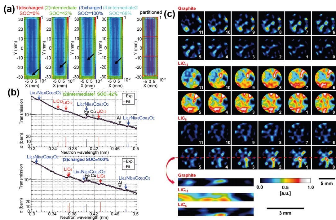
Fig. 25 (a) Transmission images of the four charge states, arrows indicate electrolyte migration. (b) Examples of the fits of the transmission spectra, with arrows indicate the positions of the Bragg edges for corresponding materials. The graph below each transmission spectrum indicates the cross section at the Bragg edge of crystalline materials on the basis of the calculation of the coherent elastic scattering. The cross sections of the graphite and \text{LiC}_6 are scaled 12 and 2 times larger, respectively. Reprinted from ref. 119 Copyright 2016, with permission from Elsevier. (c) Maps of Bragg edge heights of graphite, \text{LiC}_{12} and \text{LiC}_6 phases for horizontal (upper) and vertical slices (lower) for electrode-1 at ca. 33% SoC. The slices show an inhomogeneous distribution of the phases where black/blue represent the absence or a low proportion of the lithiation phase and red/white a high proportion. The horizontal slice number 0 was closest to the lithium-metal counter-electrode, i.e. , with increasing slice number, the distance from the Li-metal electrode. 120 Copyright 2020, CC BY.
