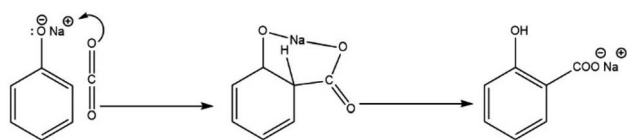
Scheme 8 Johnson's proposed intramolecular chelation mechanism.
