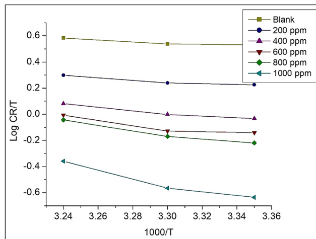
Fig. 9 Plot of log CR/T versus 1000/T for \text{Co}_3\text{O}_4 @PPy NCs.
