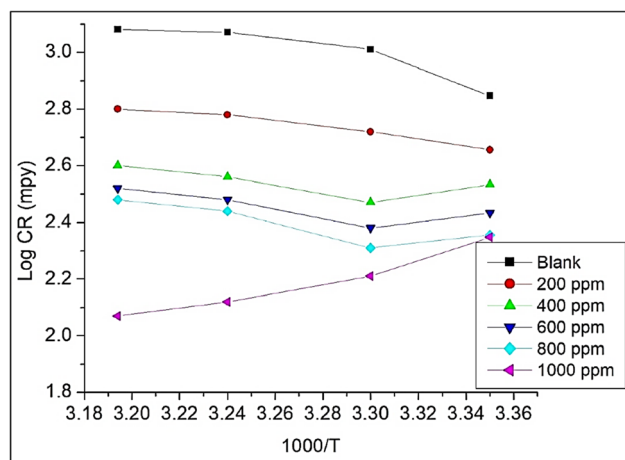
Fig. 8 Log CR (mpy) versus 1000/T for MS in \text{Co}_3\text{O}_4@PPy NCs.
