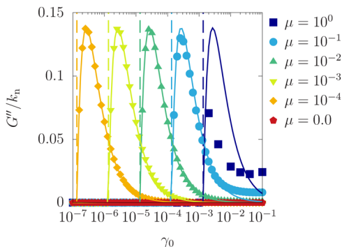
Fig. 15 Loss modulus G'' against \gamma_0 with k_t/k_n = 1.0 and \varepsilon = 0.001 for various values of \mu . The points represent the numerical results of the TBS, while the thin solid lines represent the analytical results obtained from eqn (19). The vertical dashed lines represent the critical amplitude \gamma_c(\mu) obtained from eqn (16) for \mu = 10^{-4}, 10^{-3}, 10^{-2}, 10^{-1}, 10^0 from left to right.
