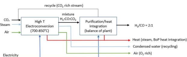
Fig. 18 Conceptual block flow diagram for the HT co-electrolysis process for syngas production.
