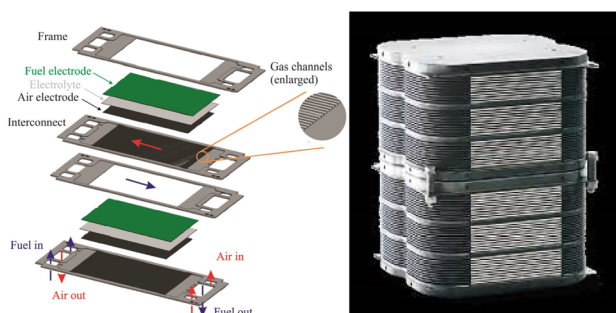
Fig. 16 Sunfire solid oxide cell and stack technology for co-SOE electrolyzers (Masini et al., 2019; Sunfire, 2022). 69,70
