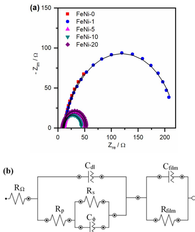
Fig. 6 (a) Nyquist plots for pristine and iron-incorporated nickel hydroxide films measured at 1.52 V vs. RHE in an alkaline medium (1.0 M NaOH) and (b) equivalent circuit employed for fitting the Nyquist plots.
