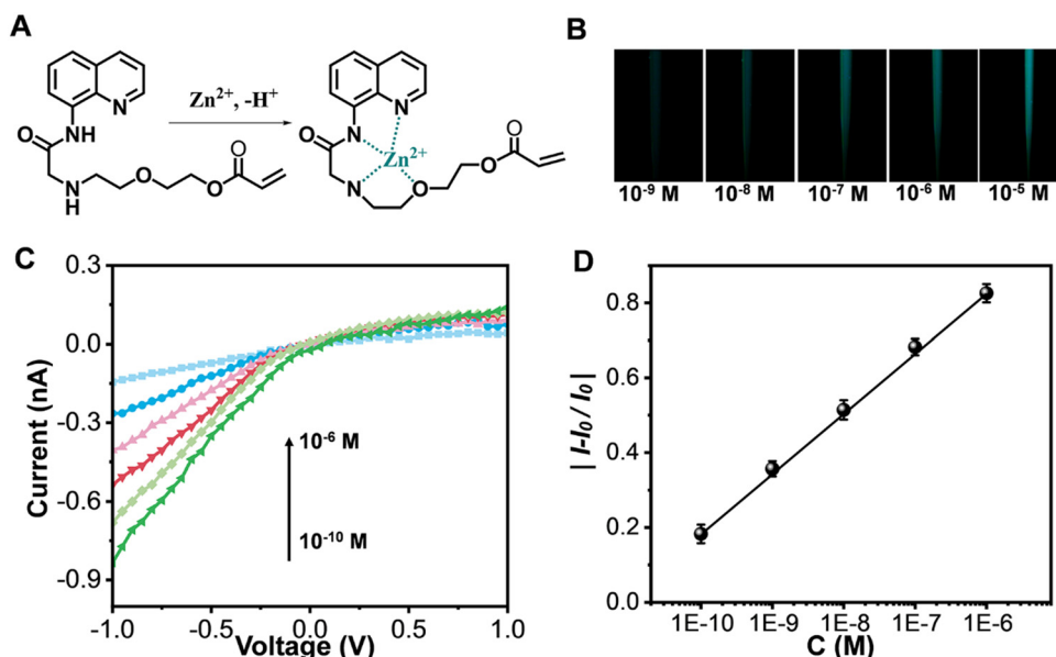
Fig. 3 (A) Chemical structure depiction of the reaction of AQZ with \text{Zn}^{2+} . (B) Fluorescence images and (C) I - V curves obtained of \text{A}\beta -copolymer-modified nanopores treated with indicated concentrations of \text{Zn}^{2+} , \lambda_{\text{ex}} = 365 \text{ nm} . (D) Calibration curve for relative current change vs. the logarithm of \text{Zn}^{2+} concentration.
