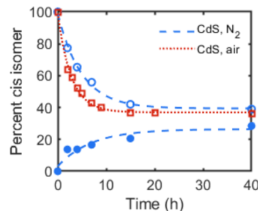
Fig. 1 Cis-trans isomerization of 3-hexene in C_6D_6 with OA-capped CdS QDs ( d \sim 2.7 nm, 1 mol%) during irradiation ( \lambda = 370 nm, 100 mW cm -2 ) plotted as percentage cis isomer over time. Open markers plot values starting from 100% trans -3-hexene at t = 0 , and shaded markers plot values starting from 100% cis -3-hexene at t = 0 . Dashed or dotted lines are exponential fits as guides to the eye.
