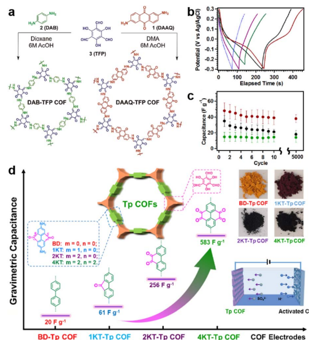
Fig. 2 (a) Synthetic routes and structures of DAAQ-TFP COF and DAB-TFP-COF. (b) GCD response and (c) average discharge capacitances at 0.1 A g^{-1} after different cycle numbers of DAAQ-TFP COF, DAAQ monomer, and DAB-TFP COF. Reprinted from ref. 29. Copyright 2013, American Chemical Society. (d) Schematic illustration, specific capacitance, and photos of Tp-COFs with different redox groups. Reprinted from ref. 41. Copyright 2020, Chinese Chemical Society.
