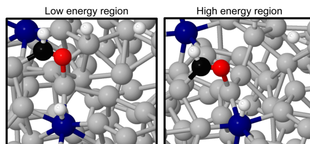
Fig. 8 A comparison of structures from the stable (left) and unstable (right) adsorption regions for liquid metal sampling of the \text{*CHO} + \text{*3H} state. The most pronounced difference is the elevation of Ga atoms underneath the adsorbates. Key: Ga-silver, Pt-blue, O-red, C-black, H-white.
