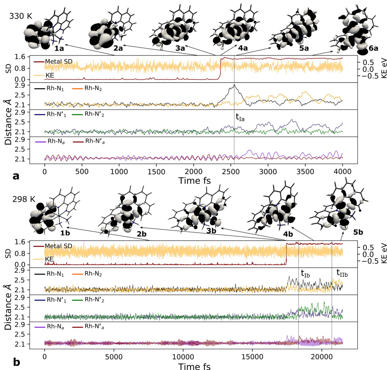
Fig. 4 Metal–ligand bond stretching of [Rh(III)(phen) 2 (NH 3 ) 2 ] 3+ (Rh – N 1 in black, Rh – N 2 in yellow, Rh – N' 1 in blue, Rh – N' 2 in green, Rh – N a in purple, Rh – N' a in red) before and after 3 LC → 3 MC crossover reaction, metal spin density (SD) and kinetic energy (KE) fluctuation at temperatures of (a) 330 K, (b) 298 K. α SOMO orbitals are plotted for several snapshots along the simulation.
