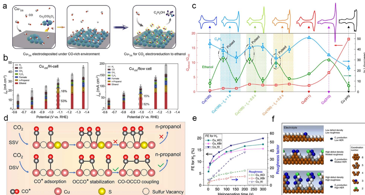
Fig. 9 (a) Schematic illustration of the synthesis of a Cu D5 catalyst under a CO-rich environment, which favours high coverage of the *CO intermediate and promotes alcohol production, and the subsequent CO 2 RR process. (b) The product distribution of the Cu D5 catalyst in an H-type cell and flow cell, respectively. Reproduced from ref. 177. Copyright 2021 Elsevier. (c) Q defects / Q 100 and product selectivity as a function of pulsed versus potentiostatic conditions on a Cu(100) electrode; copper stepped surfaces were used for comparison. Voltametric properties of the copper surfaces recorded in 0.1 M NaOH (50 mV s -1 ) are shown in the top row. Unless otherwise stated, measurements were performed at a constant potential of -1.0 V, and the pulse conditions are labelled as: E a = 0.6 V, E c = -1.0 V, t a = 1 s, t c as indicated, 1 h reaction. Measurements performed under pulsed conditions and continuous constant potential are indicated by shaded areas. Reproduced from ref. 178. Copyright 2020 Nature. (d) Schematic illustration of the formation mechanism of n -propanol on the adjacent Cu x -DSV, showing the dimerization of CO-CO and coupling of CO-OCCO. Reproduced from ref. 98. Copyright 2021 Nature. (e) Diagram of catalyst roughness and FE of H 2 as a function of halogenation time. (f) Schematic diagram of low coordination copper atoms and surface roughness with the corresponding ECR results. The coordination number for face-centred cubic copper is 12. Reproduced from ref. 180. Copyright 2020 Nature.
