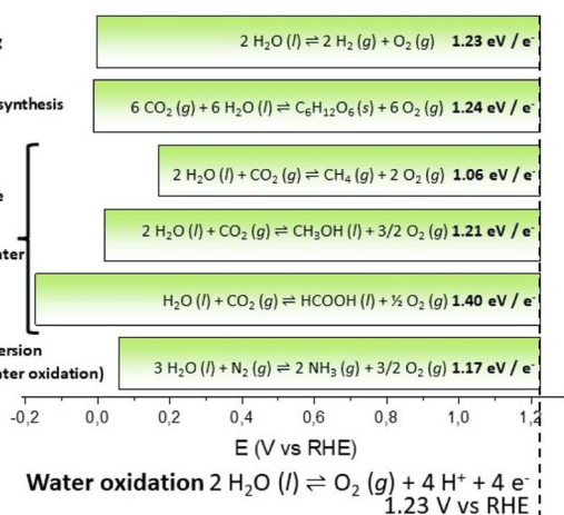
Scheme 1 Schematic representation of the energetic requirements of selected photosynthetic reactions (see eqn (1)–(6) in the main text).
