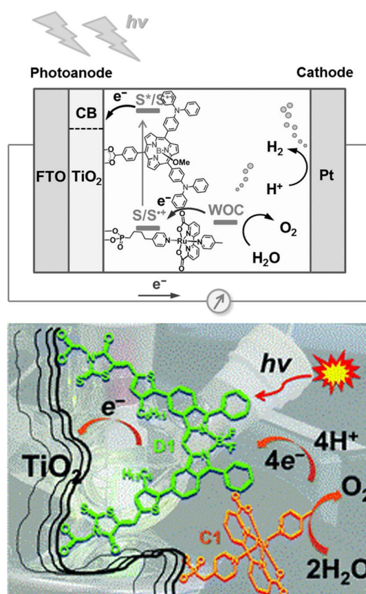
Fig. 14 Photosynthetic systems combining a Ru(bda) WOC and a subporphyrin (top) or BODIPY (bottom) photosensitizer, anchored onto a TiO 2 semiconductor. Reprinted from ref. 105 and 106 with permission from the Royal Society of Chemistry, copyright 2016 and 2017.
