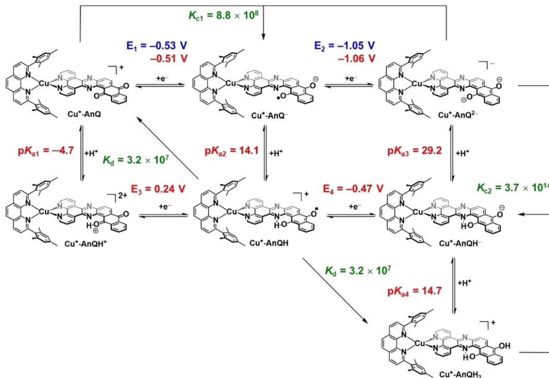
Scheme 3 Square diagram of possible protonation and reduction events starting from \text{Cu}^+\text{-AnQ} . Experimental E values in blue; calculated E and \text{p}K_{\text{a}} in red; calculated comproportionation or disproportionation values in green.
