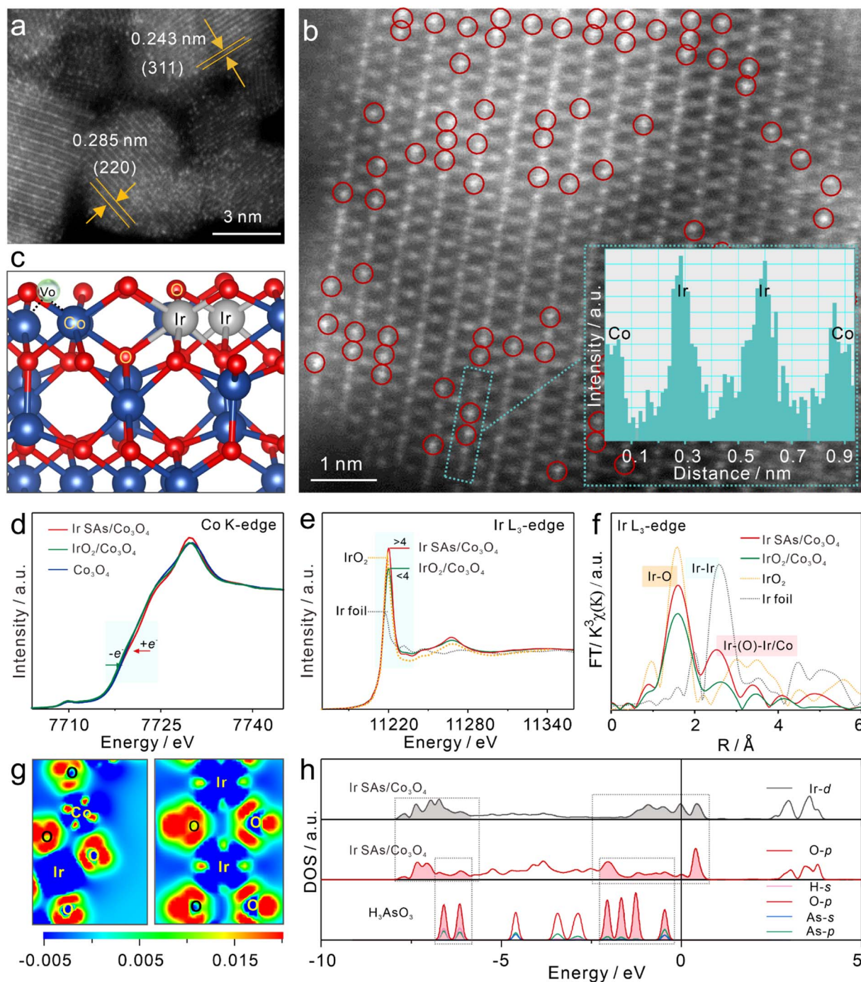
Fig. 1 Morphological and structural characterization. (a) HADDF-STEM image of Ir SAs/ \text{Co}_3\text{O}_4 collected on a randomly selected domain, where bright spots are ascribed to Ir single atoms. (b) HAADF-HRSTEM image with Ir sites marked by red circles (inset: an intensity line profile along the middle of the green dashed rectangles). (c) Side view of Ir SAs/ \text{Co}_3\text{O}_4 . Normalized XANES spectra for (d) Co K-edge and (e) Ir L_3 -edge. (f) FT-EXAFS k^3 -weighted \chi(k) function spectra (uncorrected for phase shift) for Ir L_3 -edge of Ir foil, \text{IrO}_2 , Ir SAs/ \text{Co}_3\text{O}_4 , and \text{IrO}_2/\text{Co}_3\text{O}_4 . (g) Charge density difference image on the vertical slice through the Ir, O, and Co, where blue and red regions represent the depletion and accumulation of electrons. (h) DOS of Ir and O in Ir SAs/ \text{Co}_3\text{O}_4 and free \text{H}_3\text{AsO}_3 .
