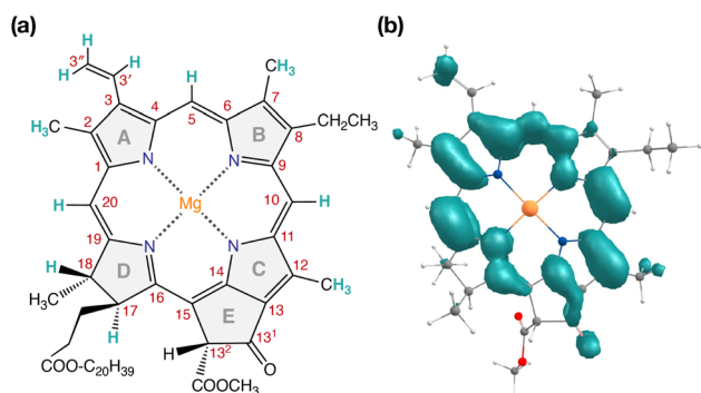
Fig. 7 (a) Structure of \text{Chl } a with carbon atom numbering and spectroscopically important hydrogen positions indicated. (b) Computed spin density distribution of triplet ( S = 1 ) \text{Chl } a .
