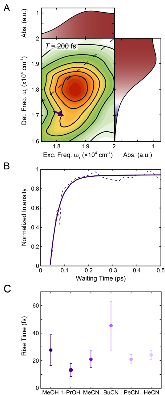
Fig. 5 (A) Reproduction of the positive region of the T = 200 fs 2DES spectrum in Fig. 1C. The purple arrow indicates the contribution from {}^1\text{MLCT} \rightarrow {}^3\text{MLCT} intersystem crossing. The corresponding linear absorption spectrum is reproduced on the top and right of the 2DES spectrum for clarity. (B) Intensity trace of the {}^1\text{MLCT} \rightarrow {}^3\text{MLCT} cross peak (dashed lines) over waiting time T along with a biexponential fit (solid lines) in methanol. See text for details. (C) Rise times of the {}^1\text{MLCT} \rightarrow {}^3\text{MLCT} cross peak (purple) in methanol, 1-propanol, acetonitrile, butyronitrile, pentanenitrile, and hexanenitrile extracted from the fits of the intensity traces (Fig. S9 and S20†). Error bars are the standard error from three replicates.
