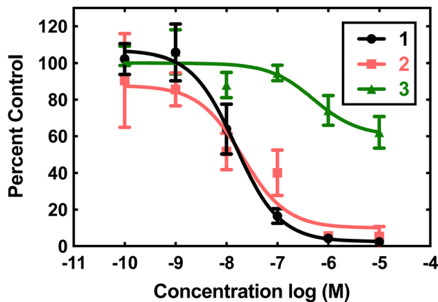
Fig. 2 Superoxide scavenging effects of 1 (black), 2 (pink), and 3 (green). \text{O}_2^{\cdot -} was generated from the reaction between hypoxanthine and xanthine oxidase reaction and detected using the chemiluminescent probe lucigenin. All reactions were carried out in pH 7.2 phosphate buffered saline (PBS) (50 mM phosphate). Data for the various concentrations of the three coordination complexes are expressed as percentages of luminescence in the presence of vehicle.
