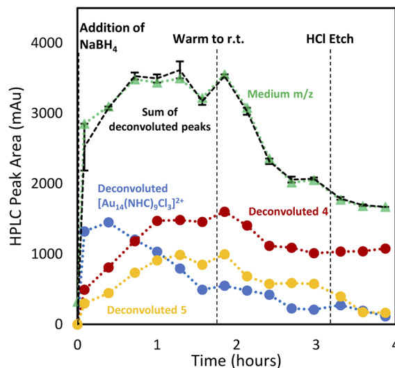
Fig. 5 Peak deconvolution of 8.5–9 min retention time window: red circle (4). Yellow circle (5), blue circle ([Au 14 (NHC) 9 Cl 3 ] 2+ ). Integrated sum for all deconvoluted signals is shown via black dashed line. Error bars indicate the difference between the sum of the deconvoluted peak fit and observed HPLC peak area (green line) for the same 8.5–9 min retention time window.
