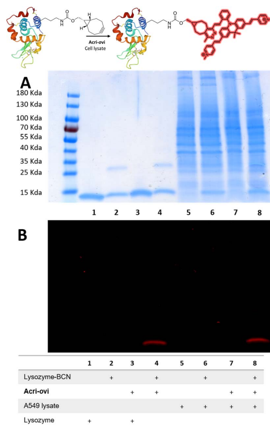
Fig. 6 Reaction of Acrid-ovi with lysozyme-BCN in the presence or absence of cell lysate. SDS-PAGE (10 \mu g per well). (A) Coomassie blue staining; (B) Fluorescence staining ( \lambda_{exc} = 496 nm).
