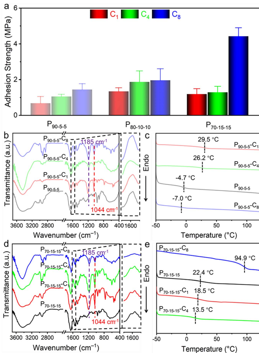
Fig. 4 Adhesion strengths of nucleobase-containing polyelectrolytes modulated through counterion exchange. (a) Adhesion strengths of P_{90-5-5} , P_{80-10-10} , and P_{70-15-15} with different counterions. (b) FT-IR spectra and (c) DSC curves of P_{90-5-5} with different counterions. (d) FT-IR spectra and (e) DSC curves of P_{70-15-15} with different counterions.
