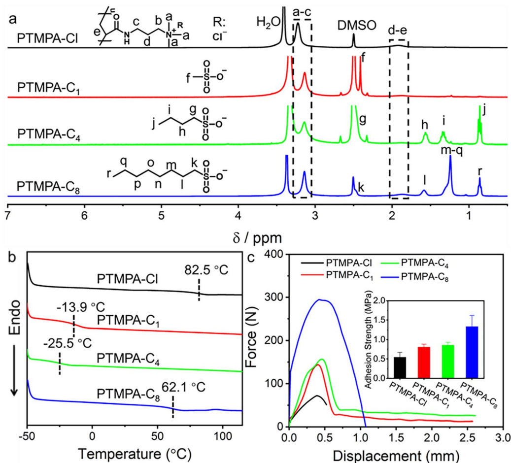
Fig. 2 Characterization of cationic PTMPAs with different counterions. (a) ^1\text{H} NMR spectra and (b) DSC curves of PTMPA-Cl, PTMPA-C 1 , PTMPA-C 4 , and PTMPA-C 8 . (c) Representative shear test curves for PTMPA-Cl, PTMPA-C 1 , PTMPA-C 4 , and PTMPA-C 8 with the inset showing the adhesion strengths.
