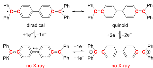
Scheme 1 Synthesis of 1 .
