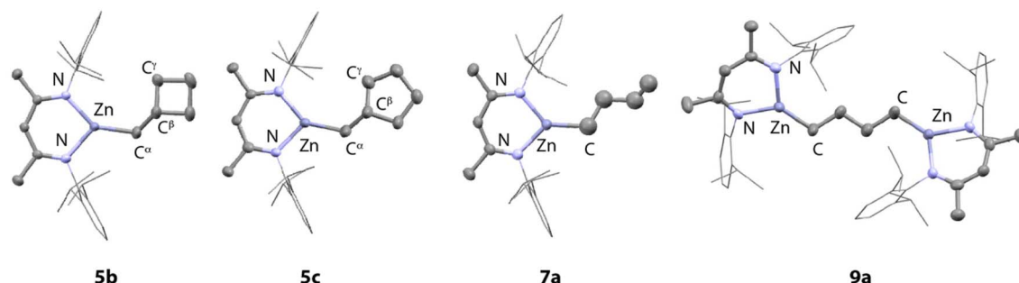
Fig. 2 Structures of 5b , 5c , 7a and 9a from single crystal X-ray diffraction experiments. Selected bond lengths (Å) and angles (°): 5b : Zn1–N1 1.9797(13), Zn1–N2 1.9554(12), Zn1–C30 1.9697(18), C30–C31 1.504(3), N1–Zn1–N2 95.86(5), N1–Zn1–C30 124.04(8), C30–Zn1–N2 140.06(8); 5c : Zn1–N1 1.9745(3), Zn1–N2 1.975(3), Zn1–C30 1.965(4), C30–C31 1.475(7), N1–Zn1–N2 95.52(11), N1–Zn1–C30 141.81(15), C30–Zn1–N2 122.56(15); 7a : Zn1–N1 1.956(2), Zn1–N2 1.964(2), Zn1–C30 1.960(3), C32A–C33A 1.157(9), N1–Zn1–N2 95.83(9), N1–Zn1–C30 131.84(10), C30–Zn1–N2 132.26(10); 9a : Zn1–N1 1.9651(16), Zn1–N2 1.9595(17), Zn1–C59 1.945(2), Zn2–N3 1.9589(17), Zn2–N4 1.9709(19), Zn2–C62 1.943(3), N1–Zn1–N2 95.47(8), N1–Zn1–C59 130.33(9), C59–Zn1–N2 134.21(8), N3–Zn2–N4 95.37(17), N3–Zn2–C62 134.54(9), C62–Zn2–N4 130.07(9).
