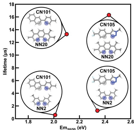
Fig. 7 Four iridium phosphor complexes and the effect of substituting the CN or NN ligand on E_{m_{50/50}} and lifetime indicated in the plot with structures shown as insets. Coordinated nitrogen (carbon) atoms are indicated with blue (gray) circles. Atoms are colored as follows: white for hydrogen, gray for carbon, blue for nitrogen, and light blue for fluorine.
