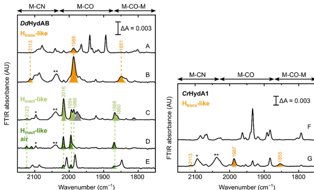
Fig. 7 Formation of the H_{trans} -like and H_{inact} -like states in WT [FeFe] hydrogenase. IR spectra of WT DdHydAB and WT CrHydA1 under several conditions. Left panel – DdHydAB : as isolated (A); with 10 mM NaCN (B); with 10 mM NaCN and 10 mM HAR (C); with 10 mM NaCN, 10 mM HAR and after exposure to air (D); after preparation of the H_{inact} state with Na_2S as described in ref. 2. Right panel – CrHydA1 : as isolated (F) and with 10 mM NaCN. Bands from the H_{trans} -like state are colored in orange, those from the H_{inact} -like state obtained under anaerobic conditions in light green and those from the H_{inact} -like state under air in dark green. The single and double asterisk indicate HCN and [Fe(CN)_6]^{4-} respectively. In (A), the additional bands (not colored) correspond to the H_{ox} and H_{red}H^+ states, with small contributions from the H_{ox}-CO and H_{red} states. A small proportion of the H_{trans} -like state is often present even in freshly-matured DdHydAB . In (C), the gray bands belong to the H_{ox}-CO state. In (D), the small blue-shift observed when the enzyme is exposed to oxygen after addition of NaCN and HAR ( H_{inact} -like air) might be caused by oxidation of the F-clusters not already oxidized by HAR. As shown in (E), the same “ H_{inact} -like air” state is routinely present as a minor component when the H_{inact} state (not colored) is prepared by addition of Na_2S and HAR, 2 as a result of the oxidation of the H_{trans} -like state formed during artificial maturation (shown in A). In (F), the additional bands belong to the H_{red} state, with smaller contributions from the H_{red}H^+ and H_{sred}H^+ states. The H_{red} and H_{sred}H^+ states are present also in (G), after addition of CN^- to CrHydA1 . Addition of CN^- to CrHydA1 seems to induce a lot more H-cluster degradation, as demonstrated by the loss in intensity in the IR spectra (while the protein concentration was similar, 420 \mu M in (F) and 500 \mu M in (G)) and the presence of an intense band for [Fe(CN)_6]^{4-} .
