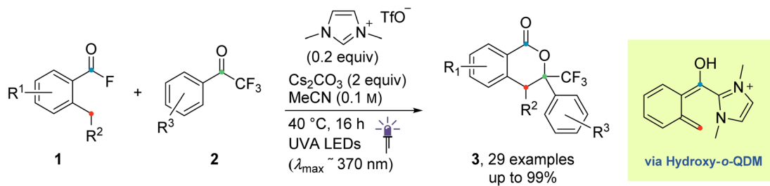
Scheme 1 The NHC-catalyzed PEDA process under investigation (previous work). 41
