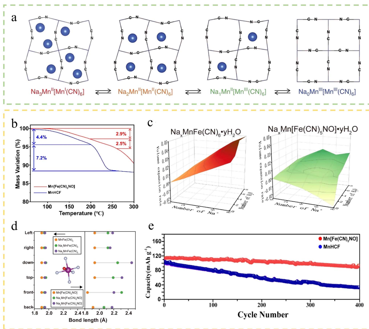
Fig. 11 (a) The schematic diagrams illustrate the changes in structure for \text{MnHCF} during battery cycling. 144 Copyright 2014, Springer Nature. (b) TG curves of \text{Mn}[\text{Fe}(\text{CN})_5\text{NO}] and \text{MnHCF} . (c) Volume change of a unit cell with different water contents during \text{Na}^+ insertion of \text{Na}_x\text{MnFe}(\text{CN})_6 and \text{Na}_x\text{Mn}[\text{Fe}(\text{CN})_5\text{NO}] . (d) Variation of manganese bond lengths with different sodium contents. (e) Cycle performance of \text{Mn}[\text{Fe}(\text{CN})_5\text{NO}] and \text{MnHCF} at a current density of 100 \text{ mA g}^{-1} . 145 Copyright 2024, Elsevier.
