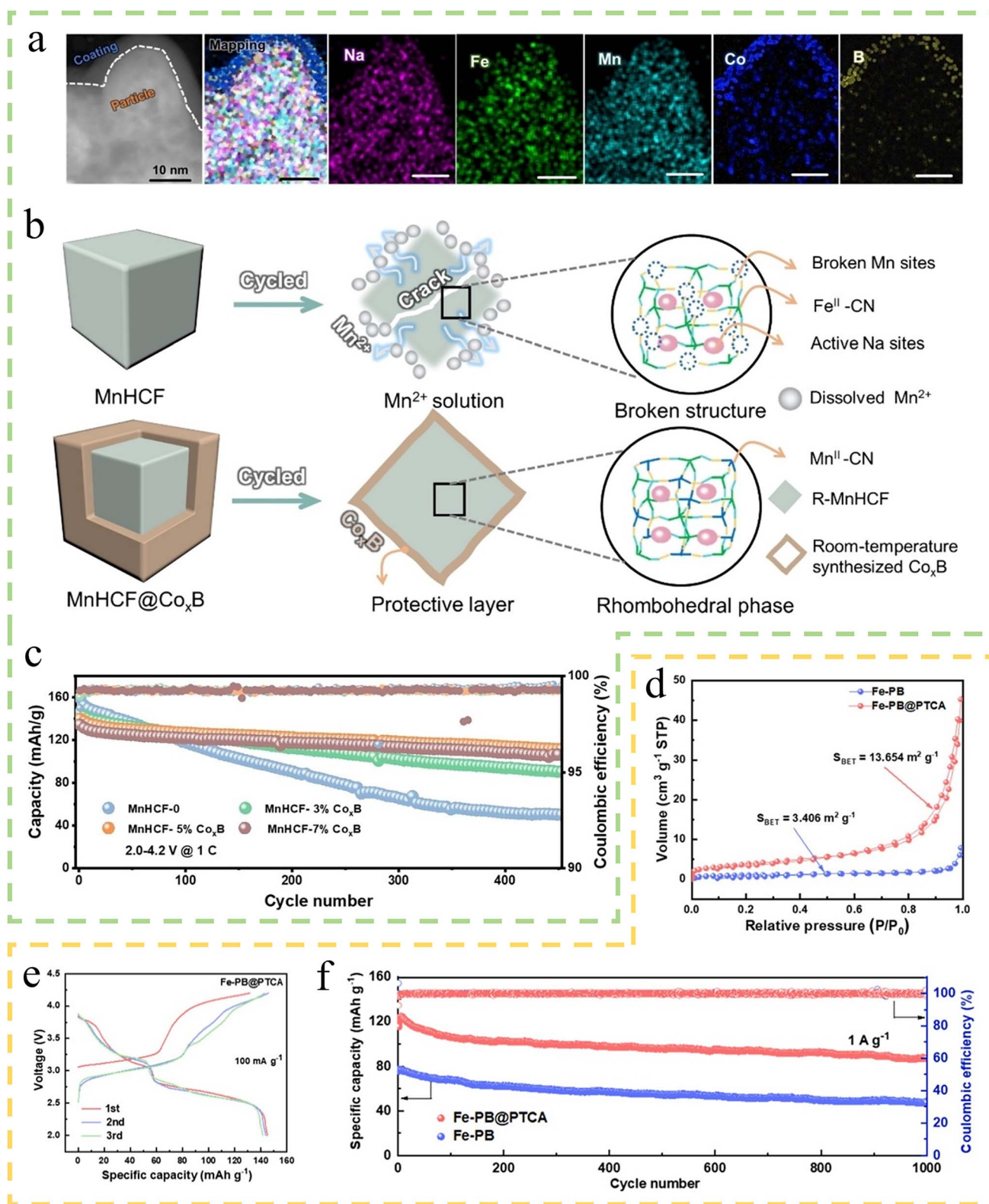
Fig. 13 (a) TEM and EDS element mapping of MnHCF-5%Co x B. (b) Schematic illustration of the proposed protective mechanism of Co x B to suppress the Mn dissolution and generation of microcracks of the MnHCF cathode. (c) The cycling stability of several electrodes at 1C. 114 Copyright 2023, Wiley-VCH. (d) N 2 adsorption-desorption isotherms of Fe-PB and Fe-PB@PTCA. (e) Charge/discharge profiles of Fe-PB@PTCA at 100 mA g -1 . (f) Long cycle performance of two samples at 1 A g -1 . 150 Copyright 2024, Wiley-VCH.
