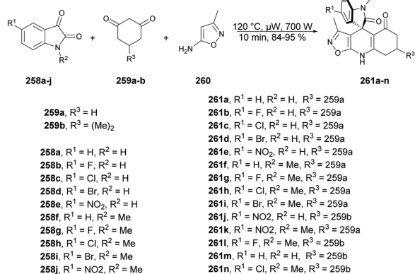
Scheme 91 Synthesis of oxazolo[5,4- b ]quinoline-fused spirooxindoles 261a–n .
