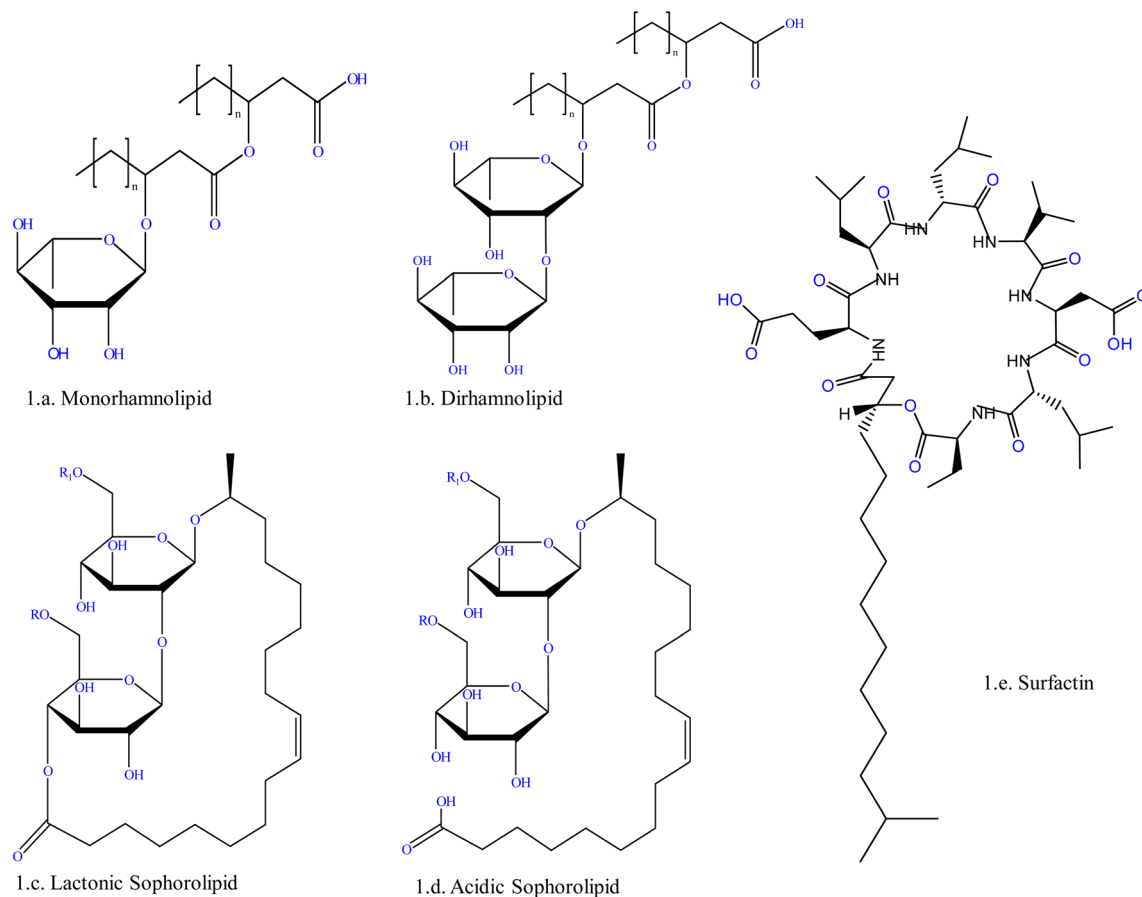
Fig. 1 (a) Monorhamnolipid. (b) Dirhamnolipid. (c) Lactonic. (d) Acidic sphorolipid. (e) Surfactin.
