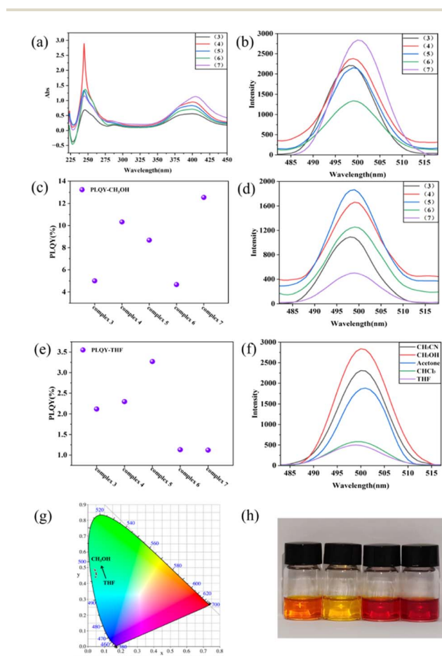
Fig. 3 (a) UV-visible spectra for complexes 3–7 in \text{CH}_2\text{Cl}_2 ( 1 \times 10^{-4} M); (b) fluorescence emissions for complexes 3–7 in \text{CH}_3\text{OH} ( 1 \times 10^{-4} M); (c) PLQY for complexes 3–7 (5.00%, 10.33%, 8.68%, 4.66%, 12.55%, respectively) in \text{CH}_3\text{OH} at room temperature ( 1 \times 10^{-4} M); (d) fluorescence emissions for complexes 3–7 in THF ( 1 \times 10^{-4} M); (e) PLQY for complexes 3–7 (2.12%, 2.30%, 3.27%, 1.13%, 1.12%, respectively) in THF at room temperature ( 1 \times 10^{-4} M); (f) fluorescence emissions for complex 7 ( 1 \times 10^{-4} M) in different organic solvents ( \text{CH}_3\text{OH} , \text{CH}_3\text{COCH}_3 , \text{CHCl}_3 , \text{CH}_3\text{CN} , THF); (g) the CIE coordinates for complex 7 ( 1 \times 10^{-4} M) from THF to \text{CH}_3\text{OH} ; (h) from left to right: color of methyl orange-sodium (1d), methyl orange-silver (2d), complex 3, complex 7 in DMF.
