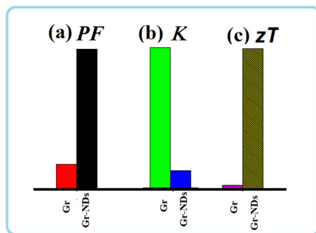
Fig. 5 Normalized (a) power factor, PF, (b) thermal conductivity, \kappa and figure of merit, zT of the Gr–NDs nanocomposite and their comparison with the values of pure graphene at RT.
