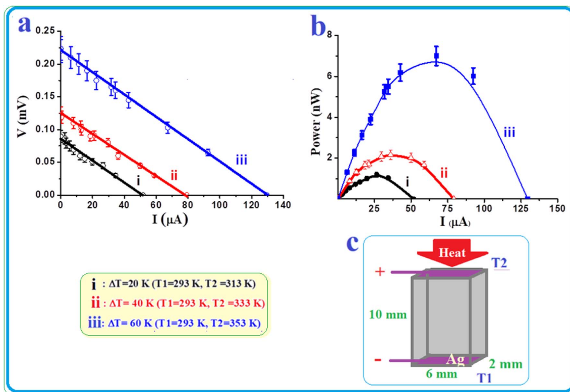
Fig. 7 Above and near RT thermoelectric power characteristics of a single leg TE module made of the Gr-NDs nanocomposite in compact rectangular form (of 2 × 6 × 10 mm) at different \Delta T values. (a) Open and closed-circuit values of V vs. I , (b) power output vs. I , and (c) dimensions of the used single-leg using rectangle-shape module.
