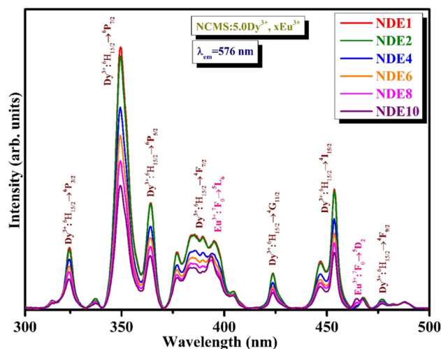
Fig. 6 Photoluminescence excitation spectra of co-activated 5.0 mol% of \text{Dy}^{3+} and x mol% of \text{Eu}^{3+} ( x = 1.0, 2.0, 4.0, 6.0, 8.0 and 10.0 mol%) \text{Na}_4\text{Ca}_4\text{Si}_6\text{O}_{18} phosphors under 576 nm emission wavelength.
