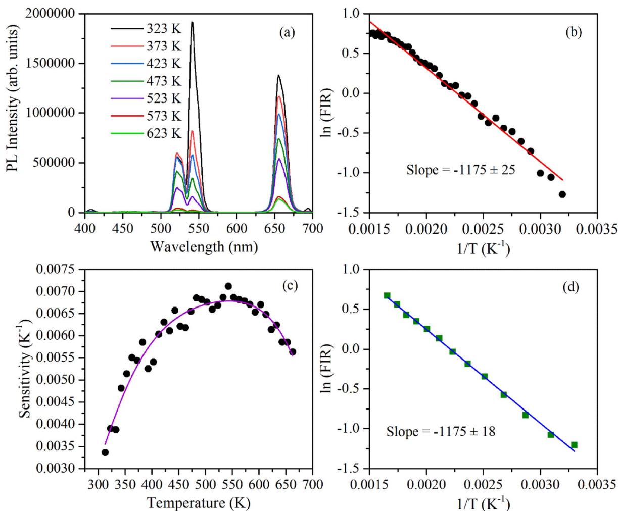
Fig. 7 UC-based ratiometric temperature sensing using \beta - \text{NaYF}_4:\text{Yb}^{3+}/\text{Er}^{3+} phosphor: (a) UC emission spectra measured between 300 and 650 K, (b) plot of \ln(\text{FIR}) (using 523 and 548 nm emission) as a function of the inverse absolute temperature during heating, (c) temperature sensitivity as a function of temperature, (d) plot of \ln(\text{FIR}) as a function of the inverse absolute temperature during cooling.
