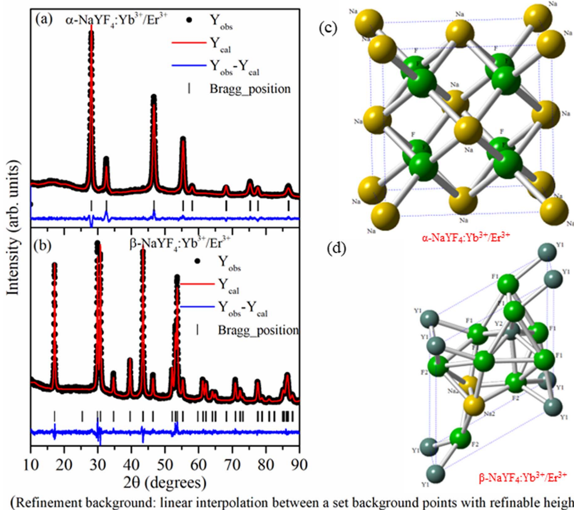
Fig. 1 Rietveld refinement of (a) \alpha\text{-NaYF}_4\text{:Yb}^{3+}/\text{Er}^{3+} and (b) \beta\text{-NaYF}_4\text{:Yb}^{3+}/\text{Er}^{3+} using Fm\bar{3}m and P_6 space group, respectively. The experimental, calculated, and difference profiles are represented by black dots, red lines, and blue (bottom) lines, respectively. Bragg reflections are denoted by vertical tick marks above the difference profile. (c) and (d) shows the crystal structure of \alpha\text{-NaYF}_4\text{:Yb}^{3+}/\text{Er}^{3+} and \beta\text{-NaYF}_4\text{:Yb}^{3+}/\text{Er}^{3+} drawn based on the Rietveld refinement data.
