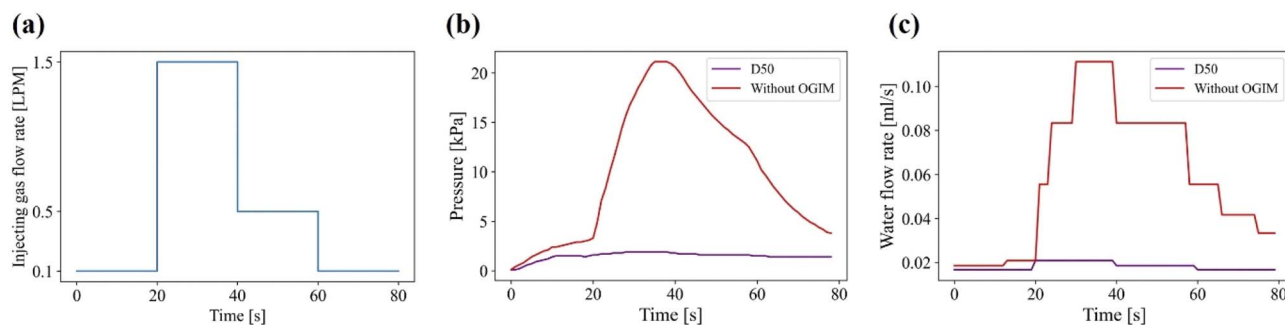
Fig. 6 Demonstration of the damping effect of the OGIM in the condition of high gas injection rate. (a) The pneumatic gas was injected into the system in the order of 0.1 LPM, 1.5 LPM, 0.5 LPM, and 0.1 LPM every 20 seconds. (b and c) The plots of the internal pressure (b) and the water flow rate (c) of the closed system without OGIM (red) and the system with OGIM-D 50 (purple).
