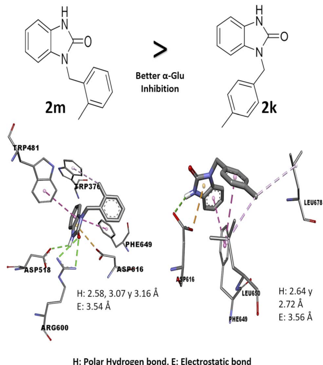
Fig. 3 Structure–activity relationship analysis of 2m and 2k compound against \alpha -glu with in silico interaction. The interaction in 2m compound shows a hydrogen and electrostatic bond with shorter distance (2.58, 3.16 and 3.54 Å) than bonds in the compound 2k (2.64, 3.72 and 3.56 Å), also, these bonds are with two catalytic amino acids.
