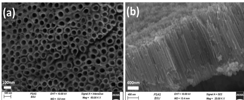
Fig. 2 Top-view (a) and side-view (b) FESEM images of TiO_2NTs photoanode.
