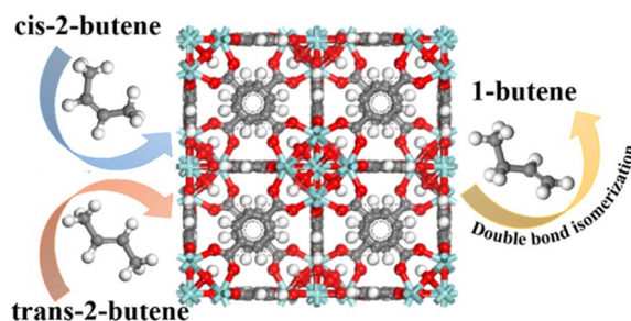
Scheme 2 The double bond isomerization of 2-butene to 1-butene.
