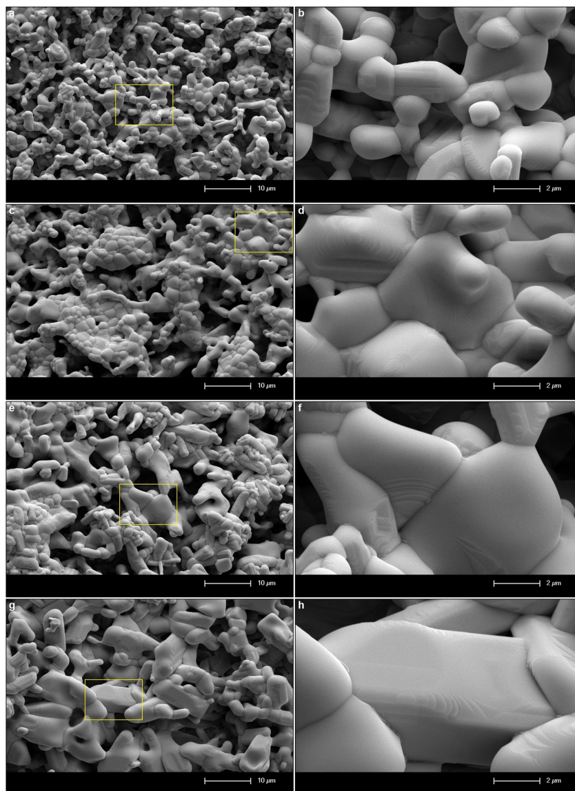
Fig. 4 SEM micrographs of 5 mol% Eu 3+ , and different concentrations B 3+ co-doped SrTa 2 O 6 samples: (a and b) without B 3+ , (c and d) 5 mol% B 3+ , (e and f) 10 mol% B 3+ , (g and h) 20 mol% B 3+ , under 15 kV accelerating voltage at 2000× and 10 000× magnifications, respectively.
