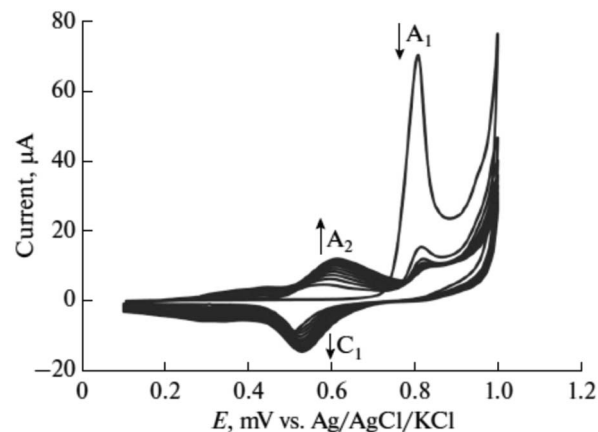
Fig. 22 Electropolymerizing process of luminol voltammogram in 0.5 M sulfuric acid under 50 mV s -1 and for 10 cycles. This figure has been adapted/reproduced from ref. 59 with permission from Springer Nature via CCC marketplace, copyright (2023).
