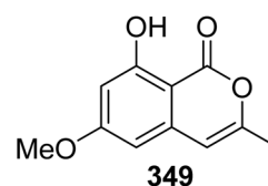
Fig. 53 Chemical structure of 349.
