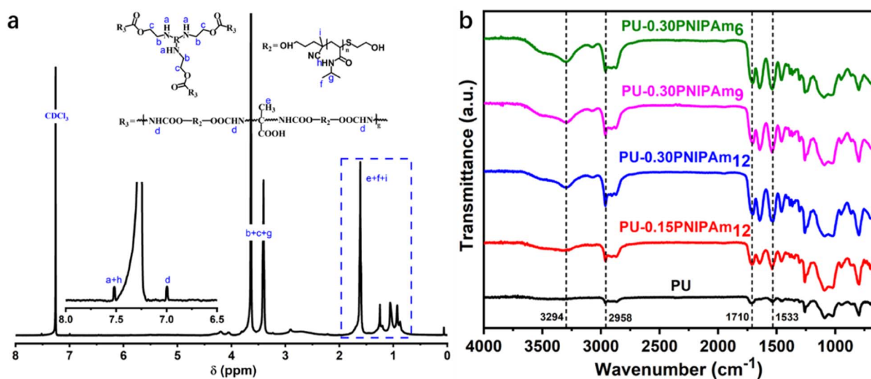
Fig. 3 (a) 1 H-NMR (CDCl 3 ) spectrum of PU-0.30PNIPAm 12 and (b) FT-IR spectrum of PU-PNIPAm n .
