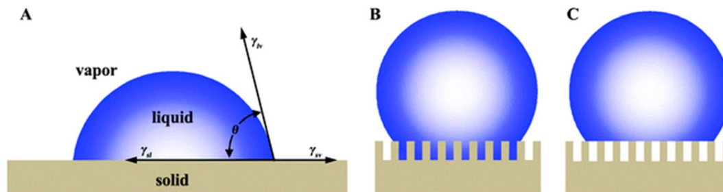
Fig. 15 Wetting behavior of solid substrates (A) Young's model (B) Wenzel's model (C) Cassie's model. Reproduced from ref. 67 with permission from Chemical Society Reviews.
