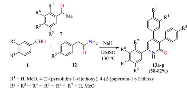
Scheme 2 One-pot three-component synthesis and anticancer evaluation of 3,4,6-triaryl-2(1 H )-pyridones 13 .
