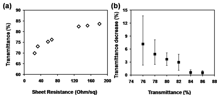
Fig. 2 (a) Plot of transmittance versus sheet resistance for CuNW transparent electrodes on N-PET substrates; (b) transmittance decrease depending on the original transparency of CuNW electrodes.
